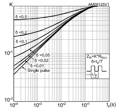
Figure 3: Thermal impedance
