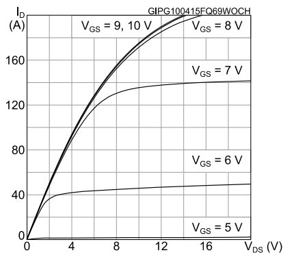
Figure 4: Output characteristics
