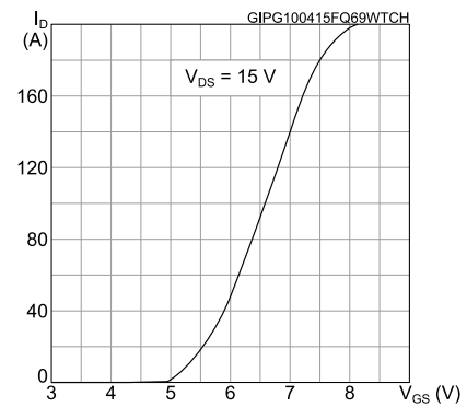
Figure 5: Transfer characteristics
