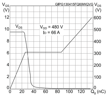
Figure 6: Gate charge vs gate-source voltage
